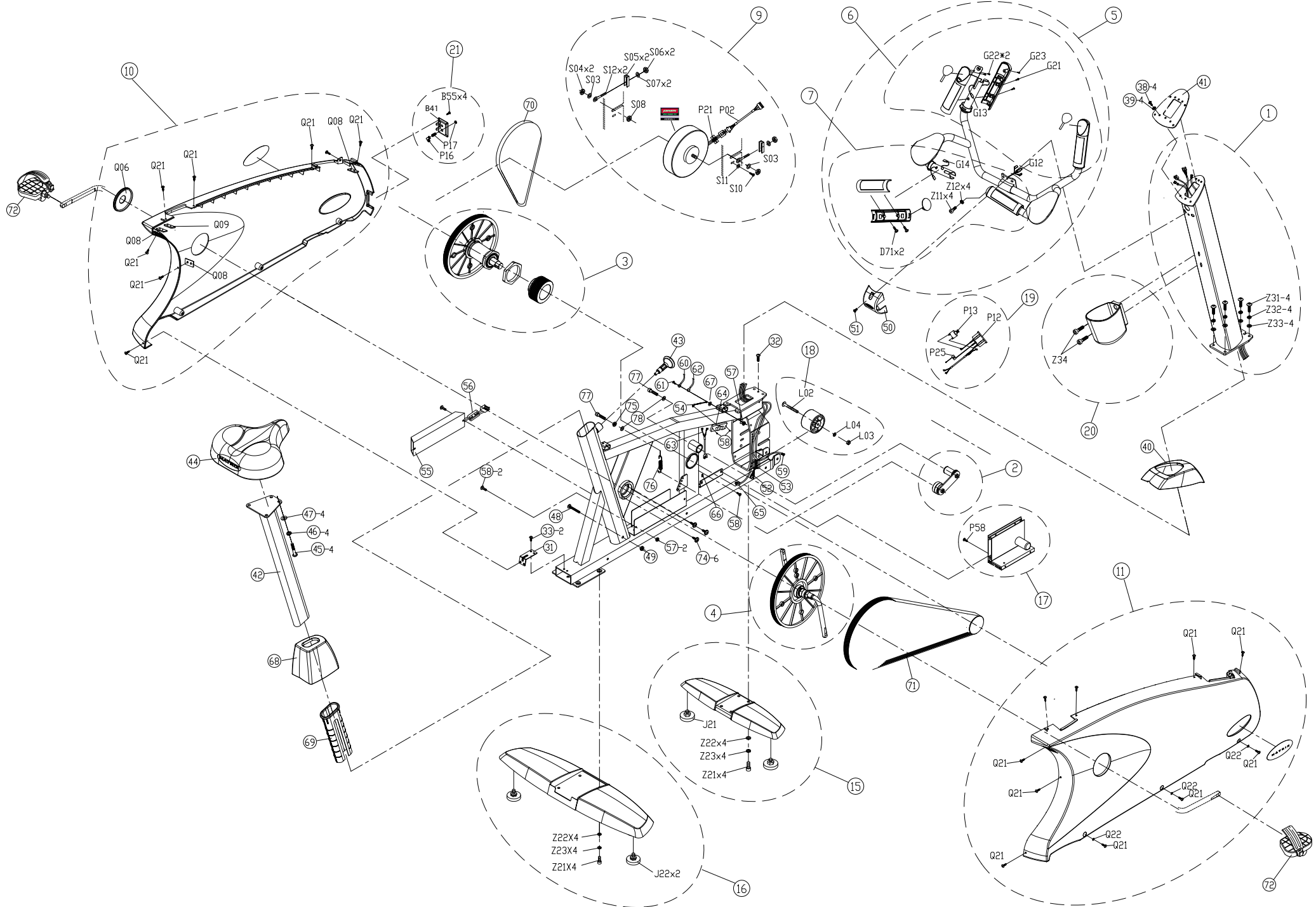
Service Drawing of Matrix U5x-F
